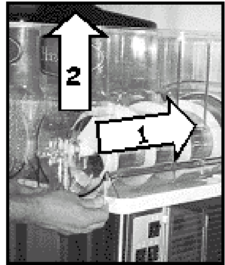
7. Remove bowl. Push in and lift up until the bowl notch clears the dispenser base.
